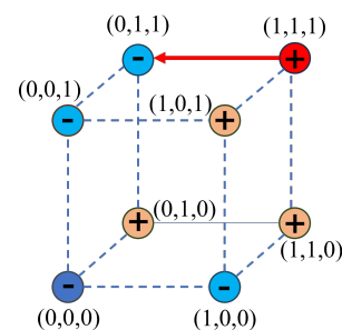
Figure 1: SEV Hypercube
