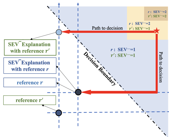
Figure 8: SEV^- distribution
