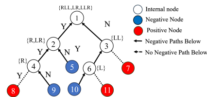
Figure 3: SEV^T Preprocessing
