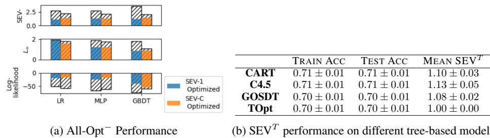
Figure 7: (a) SEV - and \ell_\infty before and after All-Opt - on the FICO Dataset. Slashed bars are before, solid color is after. (b) All tree-based models with similar accuracy have low SEV T .
