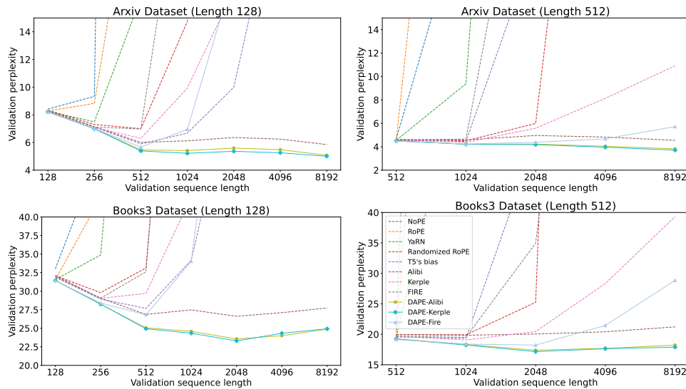
Figure 2: Comparisons with baselines: performance with training lengths 128 and 512 on Arxiv and Books3 datasets.
