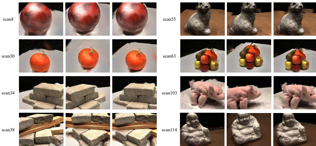
Figure 9: Examples of novel view synthesis from our method with 3 input views on the DTU dataset.
