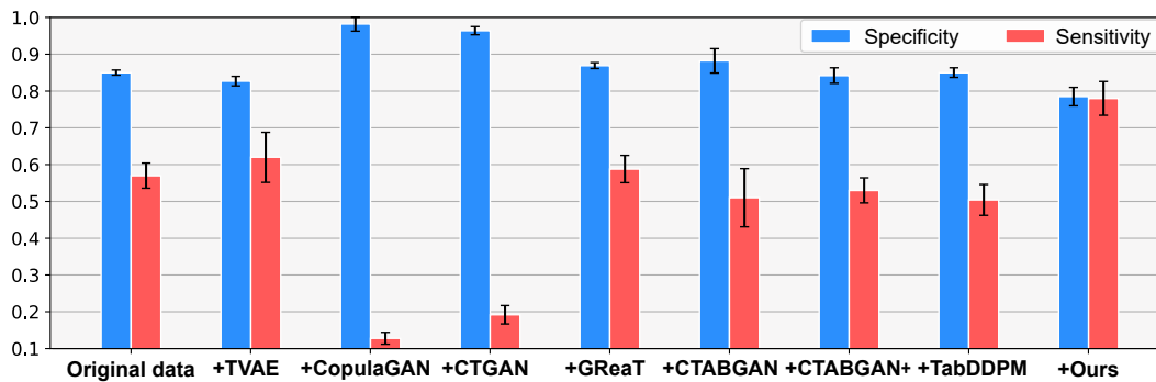
Figure 2: Comparison of ML classification performance with synthetic data on the Travel dataset. Results are averaged across four classifiers: XGBoost, CatBoost, LightGBM, and gradient boosting classifier, with each classifier run five times. Our method uses the GPT-3.5-turbo model.
