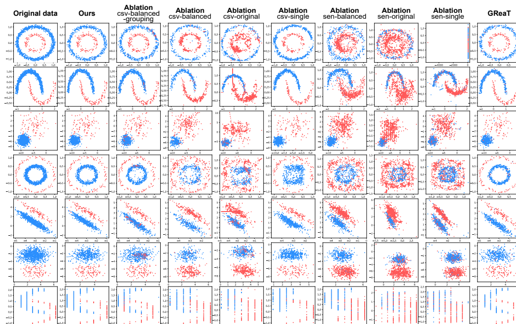
Figure 9: Complete generation results on an imbalanced toy dataset with majority and minority classes. Our approach, leveraging in-context learning with LLMs, achieves (1) distinct class boundaries, (2) accurate feature correlations, (3) well-matched value ranges, (4) robust numerical-categorical relationships (last row), and (5) comprehensive data distribution coverage, with improvements over its ablated versions and the fine-tuned GReaT model [4].
