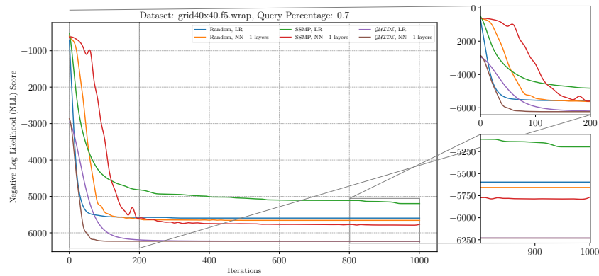
Figure 77: Analysis of ITSELF Loss Across Various Pre-Trained Models for PGMs on the grid40x40.f5.wrap Dataset at a Query Ratio of 0.7.
