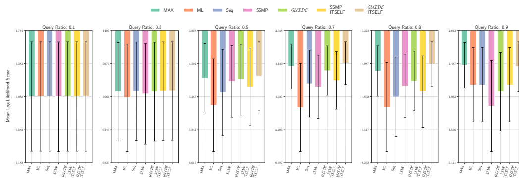
Figure 102: Log-Likelihood Scores on NLCS for PCs. Higher Scores Indicate Better Performance.
