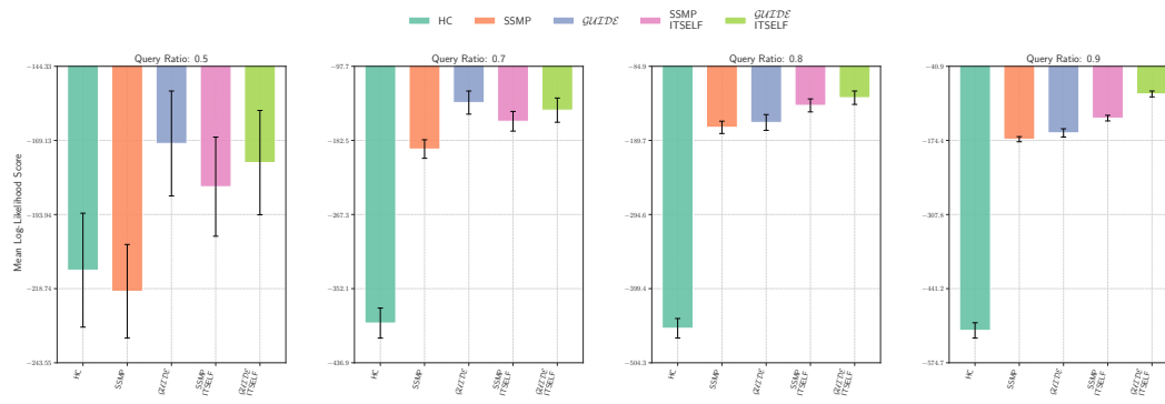
Figure 101: Log-Likelihood Scores on BBC for NAM. Higher Scores Indicate Better Performance.
