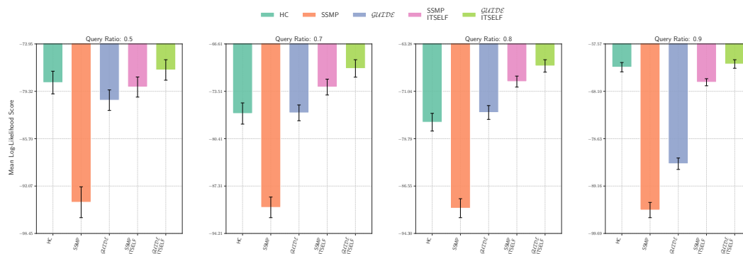
Figure 94: Log-Likelihood Scores on DNA for NAM. Higher Scores Indicate Better Performance.
