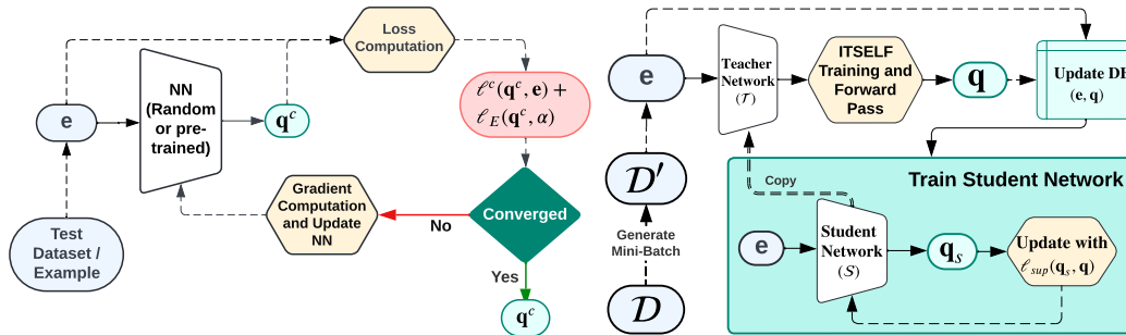
Figure 1: ITSELF Training Procedure
