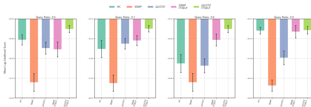
Figure 89: Log-Likelihood Scores on Accidents for NAM. Higher Scores Indicate Better Performance.
