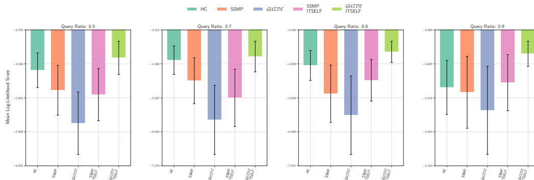
Figure 83: Log-Likelihood Scores on NAM. Higher Scores Indicate Better Performance.
