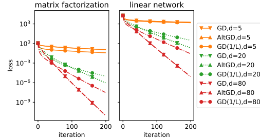
Figure 1: GD and AltGD achieve similar performance. The left plot is for (1), and the right plot is for (10).
