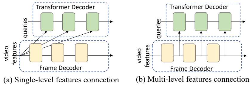
Figure 7: (a) and (b) illustrate the single-level and multi-level feature connection strategies, respectively. In (a), a single-level feature from the frame decoder is shared with the transformer decoder layers. While (b) involves the integration of multi-level features from various layers of the frame decoder. (Note: Mask inputs have been omitted for simplicity.)
