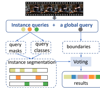
Figure 2: An efficient pipeline developed by our proposed BaFormer.
