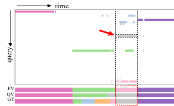
Figure 6: Query predictions and frame-wise results on 50Salads.
