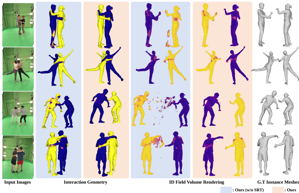
Figure C: Visualization of reconstructed multi-person interaction geometry and instance-wise volume rendering with ID fields for visualizing occluded regions during interaction.
