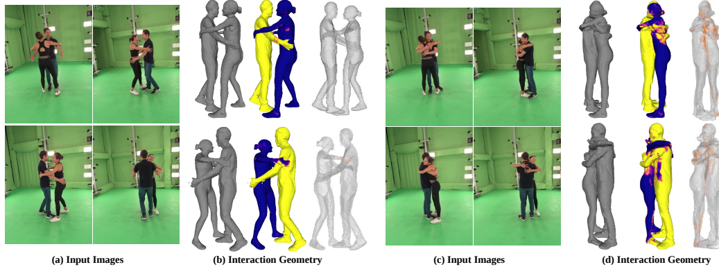
Figure I: Failure case.
