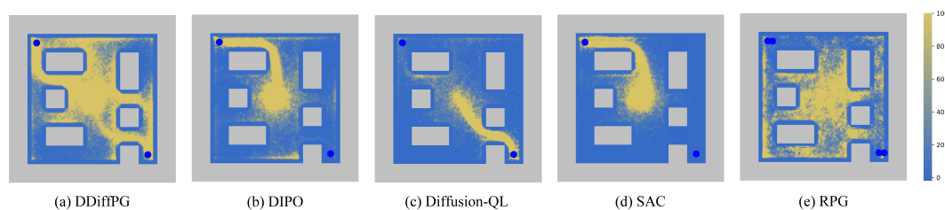
Figure 5: Exploration maps of DDiffPG and baselines in AntMaze-v3 .
