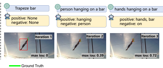
Figure 3: Illustrations of prompt optimization in a dialogue scenario. Each set shows the initial manual annotation, the subsequent prompts generated by the LLM, and the final optimized prompt that successfully guided the Vision-Language tracker to the target.
