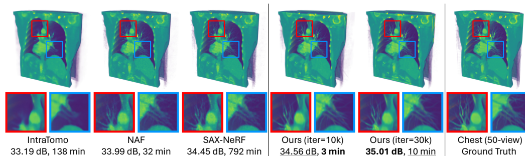
Figure 1: We compare our method to state-of-the-art NeRF-based methods (IntraTomo [66], NAF [67], SAX-NeRF [6]) in terms of visual quality, PSNR (dB), and training time (minute). Our method achieves the highest reconstruction quality and is significantly faster than other methods.
