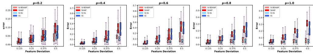
Figure 3: Evaluation results on synthetic Dataset B.
