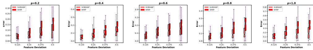
Figure 7: Evaluation results on synthetic dataset b with XGBoost.
