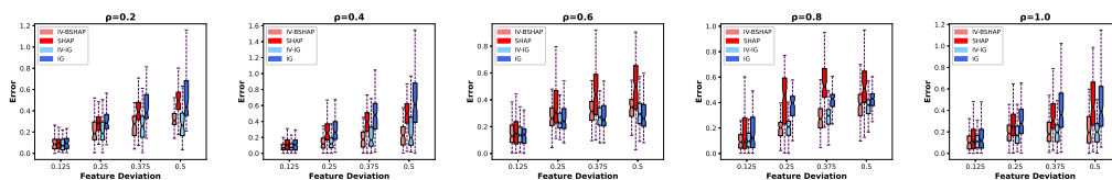
Figure 4: Evaluation results on synthetic Dataset A with DNN Classifier.
