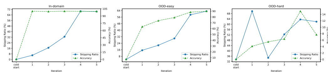
Figure 6: Skipping ratio and the accuracy of the skipping responses on Analog of Algebra.
