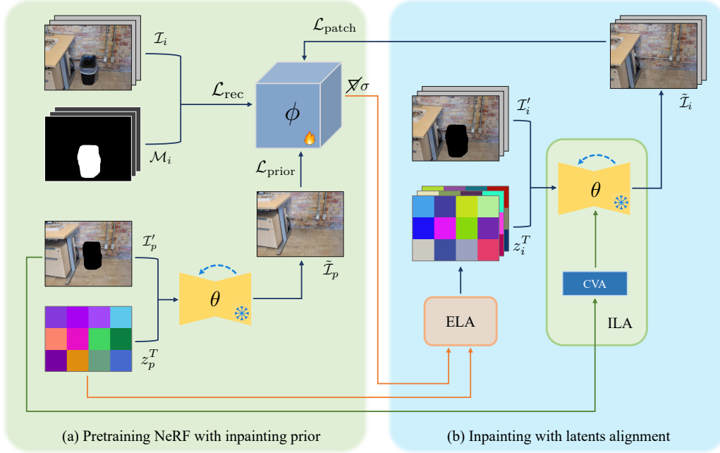
Figure 2: Overview of our method. Our approach begins with (a) pre-training the NeRF \phi with a sampled inpainting prior \tilde{I}_p from Stable Diffusion \theta , detailed in Sec. 4.1. It then progresses to (b) latent-aligned inpainting \tilde{I}_i for multi-view images through Explicit Latents Alignment (ELA) and Implicit Latents Alignment (ILA), as described in Sec. 4.2. Finally, the NeRF is optimized using a patch-based hybrid loss strategy outlined in Sec. 4.3. Throughout the training process, we fix Stable Diffusion \theta and update the scene-specific NeRF parameters \phi only.
