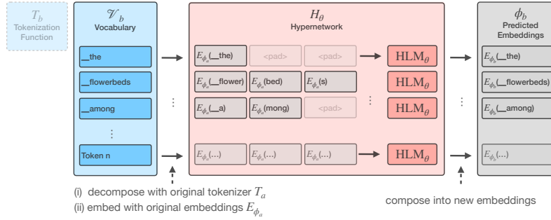
Figure 2: The hypernetwork consists of a language model HLM_\theta learning to compose embeddings under the original tokenization into a new embedding and amortizes over the tokenization function.
