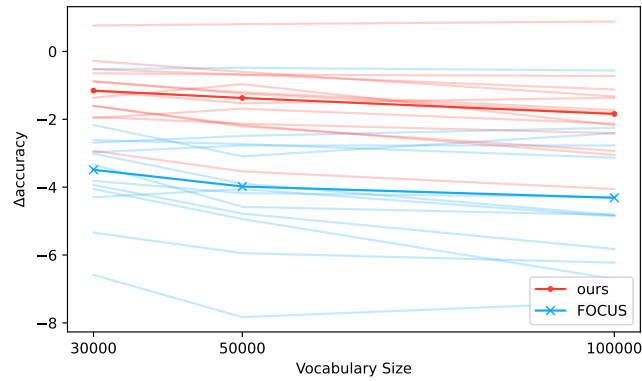
Figure 4: Difference in accuracy to the original XLM-R model on XNLI of our method and FOCUS across vocabularies with size 30k, 50k, and 100k of the new tokenizer.
