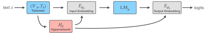
Figure 1: The hypernetwork predicts input and output embeddings based on the tokenizer.
