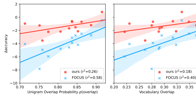
Figure 5: Correlation of the difference in accuracy to the original XLM-R model with Unigram overlap probability p(\text{overlap}) (left) and vocabulary overlap (right).
