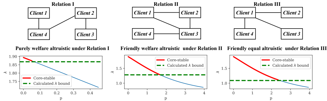
Figure 3: Partially connected: theoretically derived egalitarian fairness bounds (green dashed line) align with empirically achieved egalitarian fairness within the core-stable grand coalition (red solid line) under different client behaviors.
