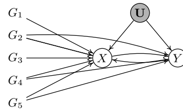
Figure 2: An illustrative example where valid and invalid IV sets induce distinct constraints, where \mathbf{G}_Y^{X \rightarrow Y} = (G_1, G_3)^\top is a valid IV set, while \mathbf{G}_X^{Y \rightarrow X} = (G_2, G_4, G_5)^\top is invalid due to pathways G_2 \rightarrow Y , G_4 \rightarrow Y and G_5 \rightarrow Y .
