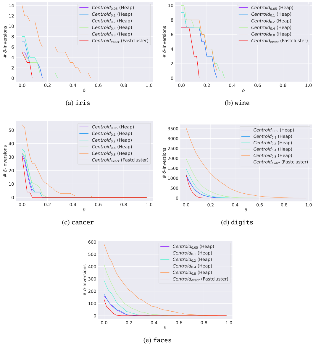
Figure 5: Non-Monotonicity of Centroid HAC: No. of \delta -inversions vs \delta
