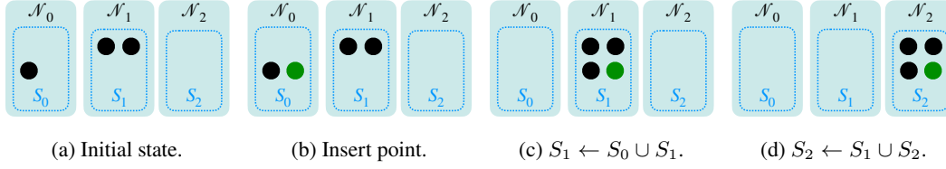
Figure 3: Our merge-and-reduce strategy when a point (in green) is inserted.
