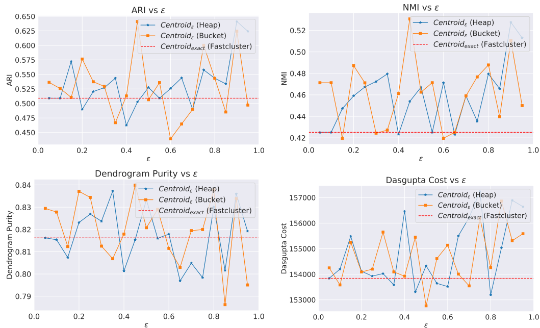
Figure 8: Quality Evaluations of the cancer dataset
