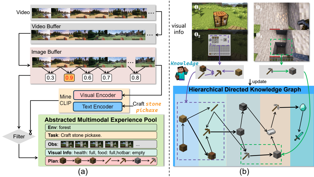
Figure 2: (a) Extraction process of multimodal experience. The frames are filtered through video buffer and image buffer, then MineCLIP [7] is employed to compute the visual and sub-goal similarities and finally they are stored in Abstracted Multimodal Experience Pool. (b) Overview of Hierarchical Directed Knowledge Graph. Knowledge is stored as a directed graph, where its nodes represent objects, and directed edges point to materials that can be crafted by this object.
