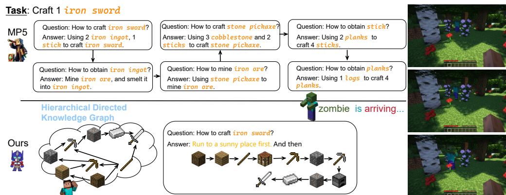
Figure 13: In this example, a zombie is slowly approaching the agent. Agents like MP5 [33] and Voyager [47] uses an iterative planning strategy to generate the plan, which consumes a great deal of time and puts the agent in danger. While Optimus-1 directly generates a plan in one step based on the knowledge graph. Using the current visual information, it makes a plan to "run to a sunny place," allowing the agent to avoid danger then begin to achieve sub-goals.
