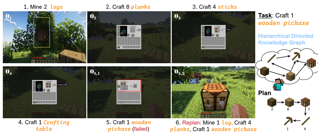
Figure 9: The process of completing the task "Craft 1 wooden pickaxe". Optimus-1 gives wrong planning. When Optimus-1 realizes it cannot complete the task, it will replan the current task.
