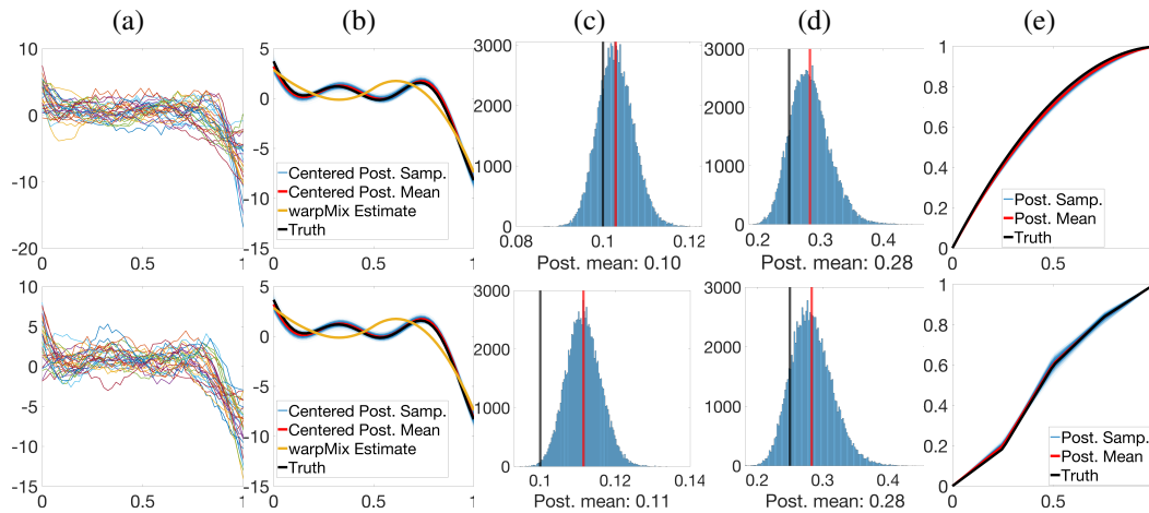
Figure 2: Row 1: Phase functions from PM1. Row 2: Phase functions from PM2. (a) Simulated data ( n = 30 ). (b) Estimation of \mu : ground truth (black), posterior samples (blue), posterior mean (red), warpMix estimate (yellow). (c)&(d) Histograms of posterior samples for \sigma^2 and \sigma_c^2 , respectively (posterior mean in red; ground truth in black). (e) Estimation of phase function for a randomly chosen observation: ground truth (black), posterior samples (blue), posterior mean (red).
