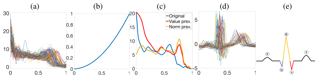
Figure 1: (a) Berkeley growth rate curves. (b) Convex phase function \gamma . (c) One example function f from (a) (blue) transformed by value-preserving action f \circ \gamma (red) and norm-preserving action (f \circ \gamma)\sqrt{\gamma} (yellow). Here, f \circ \gamma has the same classical notion of shape as f , whereas (f \circ \gamma)\sqrt{\gamma} has the same size-and-shape as f as described in Section 2. (d) PQRST complexes. (e) PQRST pattern: P wave (first max), QRS complex (sharp min-max-min) and T wave (last max) [Pham et al., 2023].
