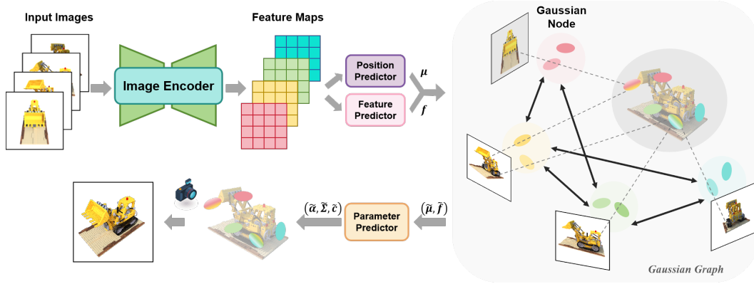
Figure 2: Overview of Gaussian Graph Network. Given multiple input images, we extract image features and predict the means and features of pixel-aligned Gaussians. Then, we construct a Gaussian Graph to model the relations between different Gaussian nodes. We introduce Gaussian Graph Network to process our Gaussian Graph. The parameter predictor generates Gaussians parameters from the output Gaussian features.
