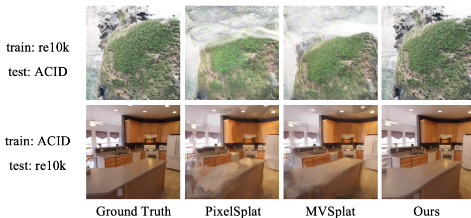
Figure 5: Visualization of model performance for cross-dataset generalization on RealEstate10K [64] and ACID [24] benchmarks.
