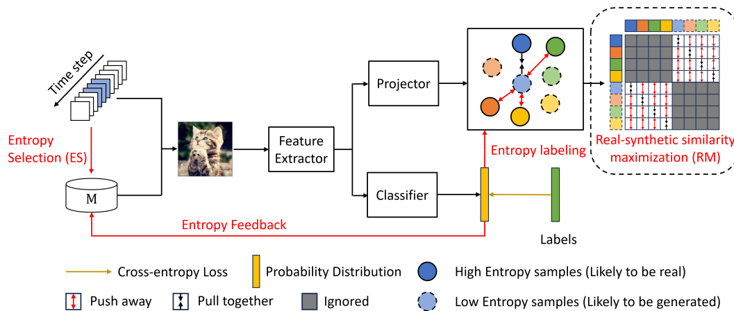
Figure 1: Overview of proposed ESRM framework for online CL. The proposed ESRM framework has two main components: Entropy Selection (ES) and Real-synthetic similarity Maximization (RM). Motivated by Obs. 2 and Obs. 3, ES is a buffer management strategy designed to use entropy as a criterion to select more real samples in the memory buffer, thereby alleviating catastrophic forgetting and performance degradation caused by the contamination. RM aims to bridge the embedding gap between synthetic and real data, as noted in Obs. 4, using a contrastive learning technique.
