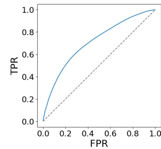
Figure 7: The ROC curve of the model trained with ESRM on the In-100/SDXL dataset ( P = 50\% ) in predicting the synthetic status of samples in the training dataset. Real samples are regarded as positives and synthetic samples as negatives.
