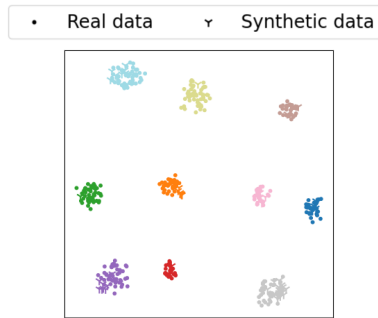
Figure 5: T-SNE visualization of memory data produced by ESRM at the end of training on the In-100/SDXL ( P = 50\% ) dataset. For clarity, only the first 10 classes are visualized.
