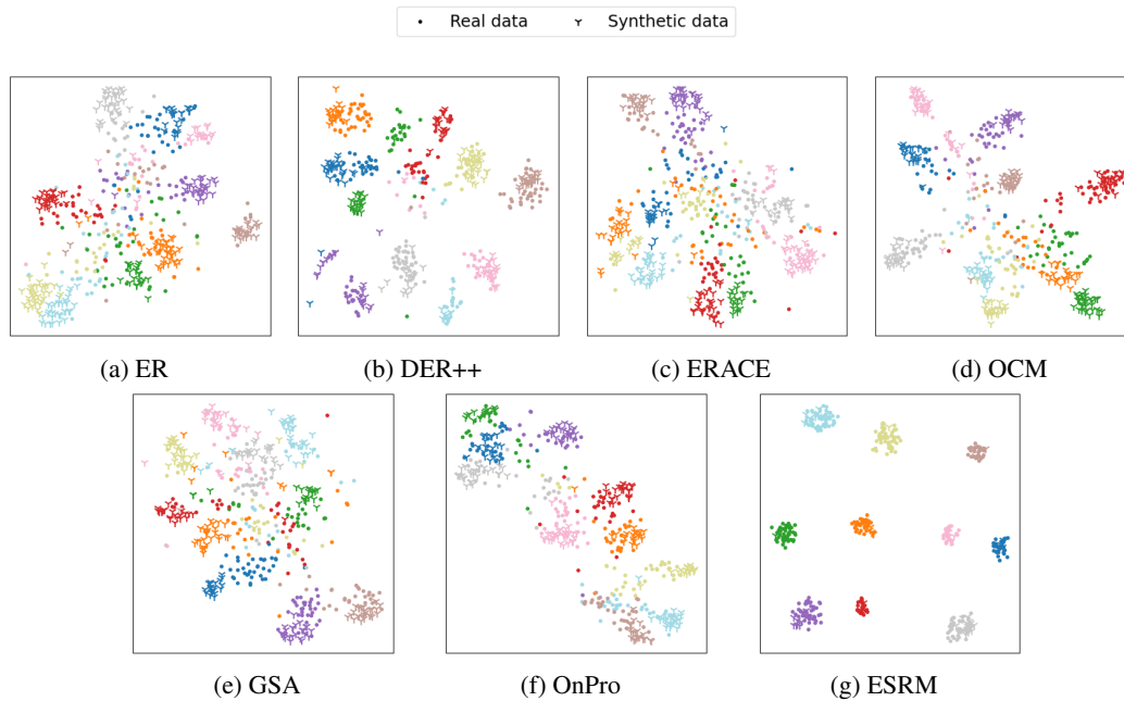
Figure 9: T-SNE visualization of the memory data at the end of training on In-100/SDXL ( P = 50\% ). For clarity, only the first 10 classes are visualized.
