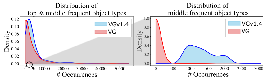
Figure 9: The large discrepancy between DeiVG and standard Visual Genome. DeiVG uses Visual Genome with extended annotations (VG v1.4 ), but the older version (VG) (Krishna et al., 2017) has been commonly used for SGG training. Object types are sorted w.r.t. the number of occurrences (x-axis) and their corresponding occupancies are shown (y-axis). The left plot is for top-and-middle frequent object types (0-50k #occ.), and the right plot is for middle frequent object types (0-3k #occ.). VG v1.4 contains many object types that do not appear in VG (Best viewed in color).
