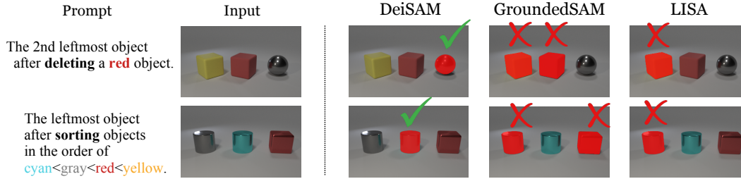
Figure 6: DeiSAM performs abstract reasoning segmentation. When presented with a visual scene paired with an abstract, complex prompt (left), DeiSAM effectively identifies and segments the object specified by the prompt, while neural baselines frequently fail to deduce the target object (right).
