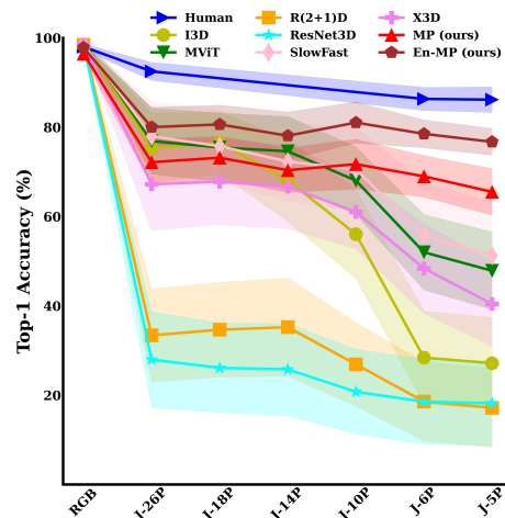
Figure 4: Our model demonstrates human-like robustness under reduced visual information. Top-1 action recognition accuracy is a function of the number of points (P) in Joint (J) videos. Results from RGB test videos are at the leftmost. The colored shaded region represents the standard error across all action classes.
