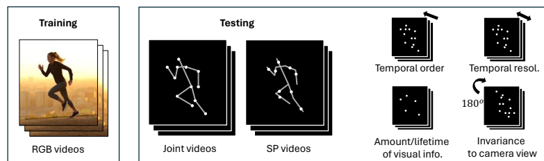
Figure 1: Humans excel at biological motion perception (BMP) tasks with zero training, while current AI models struggle with poor generalization performance. AI models are trained to recognize actions from natural RGB videos and tested using BMP stimuli on point-light displays, which come in two forms: Joint videos, which display only the detected joints of actors in white dots, and Sequential position actor videos (SP), where light points in white are randomly positioned between joints and reallocated to other random positions on the limb in subsequent frames (Sec. 3.1). Note that skeletons, shown in gray in the example video, are not visible to humans or AI models during testing. The generalization performance of both humans and models is assessed after varying five properties in temporal and visual dimensions. See Appendix, Sec. A.1 for example videos.
