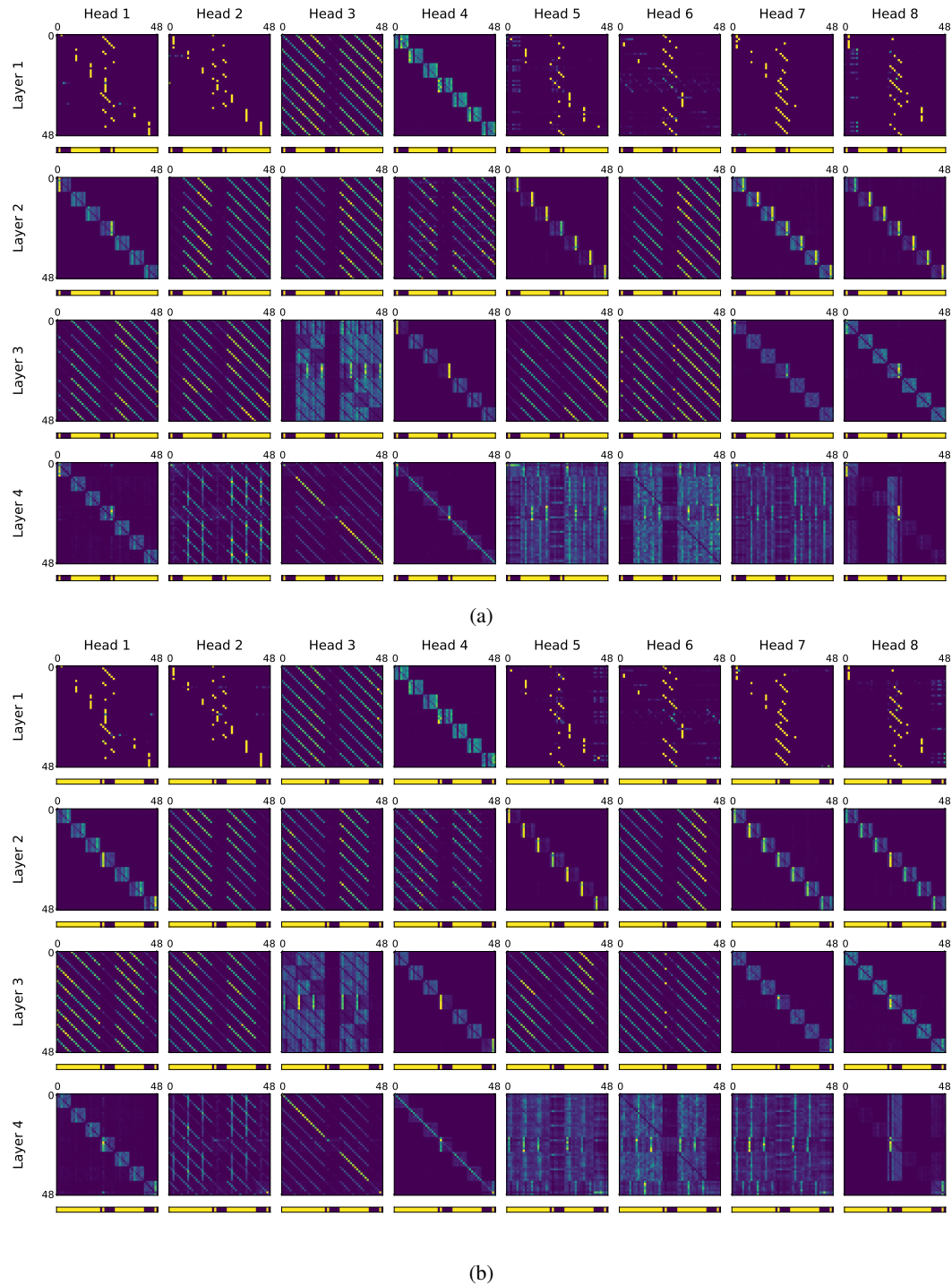
Figure 23: Attention heads and corresponding masks; blue denotes masked position in the input matrix.
