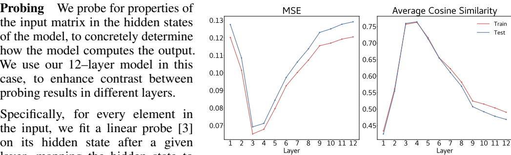
Figure 6: Hidden states encode input information. We probe for the row of each element in the masked matrix input, replacing missing entries by 0. We find that layers 3 and 4 have a much lower MSE and a much larger cosine similarity compared to other layers in the model. Hence, these layers somehow ‘store information’ about the masked input matrix.
