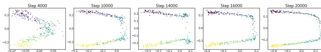
Figure 9: Token embedding structure appears before sudden drop. Projection of token embeddings along principal components of embeddings at step 50000. (Labels same as Fig. 7). Embeddings align with the principal components early on in training before the sudden drop in loss.
