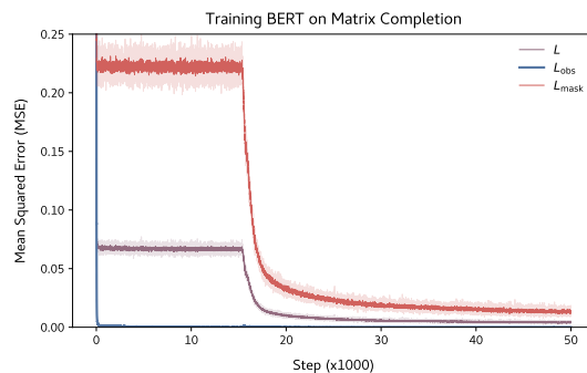
Figure 2: Sharp reduction in training loss.
