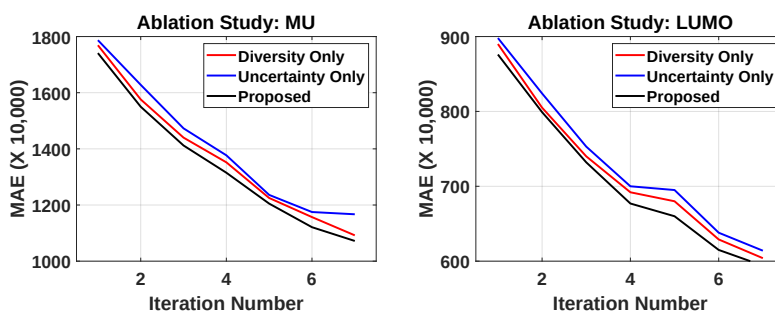
Figure 10: Ablation study results studying the individual impact of uncertainty and diversity on the mu and lumo properties with SphereNet. Best viewed in color.
