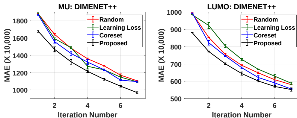
Figure 8: Study of our framework using the DimeNet ++ backbone. The graphs show the mean (averaged over 3 runs) and the errorbars for all the methods. Best viewed in color.
