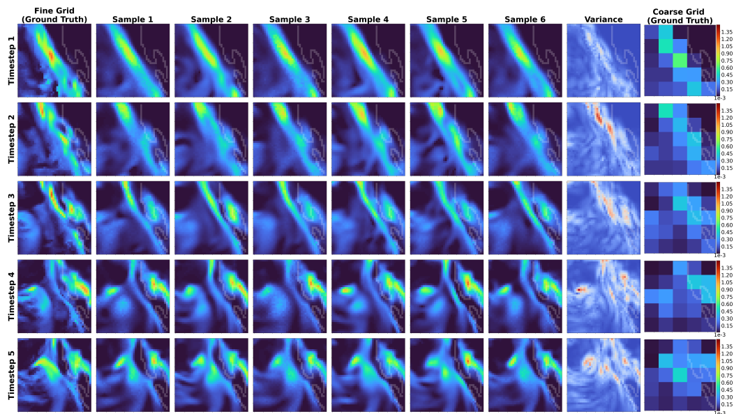
Figure 7: A visualization of the stochastic samples predicted by STVD for a given coarse-grid data. The precipitation event is the same as depicted in Fig. 3. Additionally, we also plot a variance map over the set of these samples to analyze the stochasticity better. Red regions correspond to high variance whereas blue regions correspond to low variance. Model stochasticity seems to be meaningful since the variance is large where mean precipitation is large.
