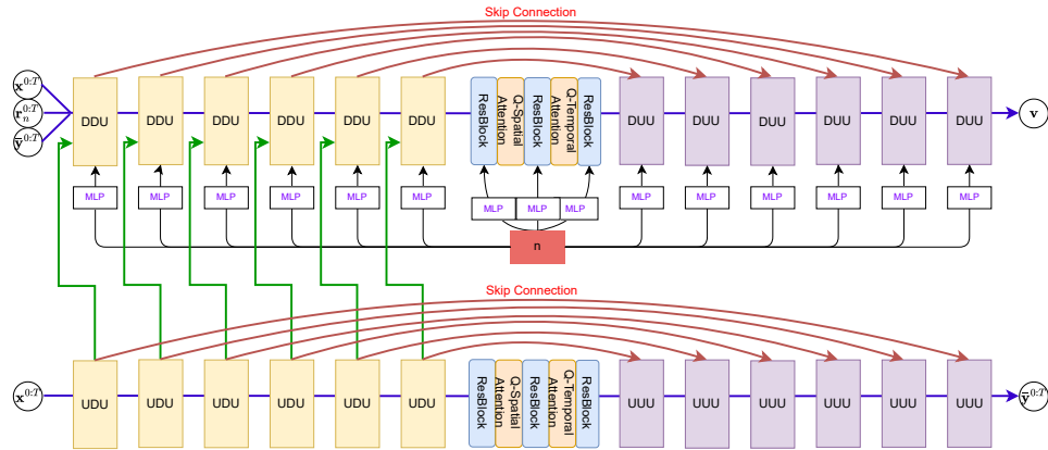
Figure 8: The figure depicts the overall model architecture where the top UNet performs diffusion on the residual, conditioned on the noise step n , \mathbf{x}^{0:T} , \mathbf{y}^{0:T} and the context of the bottom U-Net feature map (refer to Eq. (1) in Sec. 2.1). The bottom UNet is the deterministic downscaler. Details of each block are shown in Figure 9.
