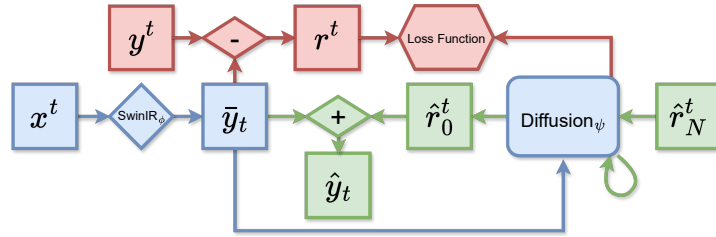
Figure 10: An illustration of the training and inference pipelines of Swin-IR-Diff. Similar to Fig. 2, blue blocks represent operations common to both training and inference phases. Red blocks signify operations exclusive to training, while green blocks indicate inference-only processes. However, in contrast, it is an image-only downscaler. This model takes in a current low-resolution frame which is deterministically downscaled via Swin-IR, followed by modeling of the residual details via conditional diffusion. The model details remain similar to what is described in A.1 with the absence of downscaler-conditioning and temporal attention in the diffusion model.
