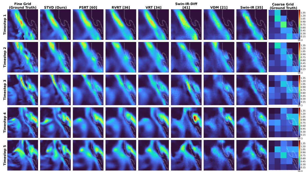
Figure 3: A qualitative comparison between our proposed model and top baseline for a precipitation event associated with a cold front impinging on the Northern California coast and then the Sierra mountain range (coastline marked in hazy white). Fig. 6 plots the regional topography. The time interval between adjacent frames is 3 hours; the plotted region is 1000 \times 1000 km. Our model resolves the fine-grid precipitation structure better than the considered baselines. See A.3 for full-page high quality samples from Himalayas and Sierra.
