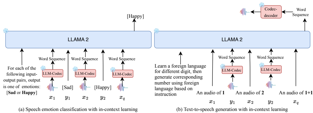
Figure 1: This figure illustrates the framework of the proposed approach (UniAudio 1.5) for performing speech emotion classification and simple text-to-speech generation tasks. For each task, we prepare the instruction, demonstrations (e.g., \{x_1, y_1, x_2, y_2\} ), and the query x_q . The LLAMA 2 model is then asked to predict the corresponding result y_q . Here, y_q can be either text or audio.
