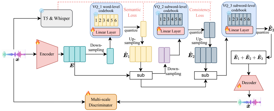
Figure 2: This figure provides a high-level overview of LLM-Codec, including an encoder, a decoder, a multi-scale discriminator, and multi-scale residual VQ layers. Here, ‘sub’ denotes feature subtraction. Note that the modules marked with a snowflake are frozen during training.
