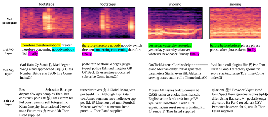
Figure 6: The token visualization of three VQ layers with LLM-Codec. The audio samples are from the ESC50 dataset.
