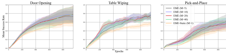
Figure 6: Ablation study on the max reward scaling M ( M = 1, 5, 10, 20, 40 ).
