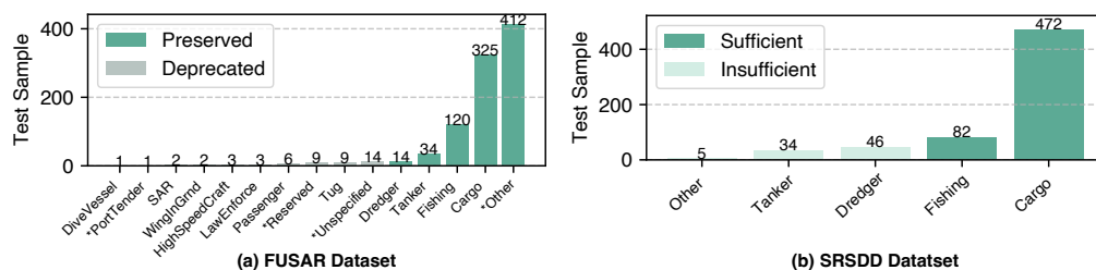
Figure A1: Constraints of the SAR datasets’ test sets. This figure illustrates the per-category test sample distribution of (a) the FUSAR dataset and (b) the SRSD dataset. The FUSAR dataset suffers from insufficient test samples and vaguely defined classes (indicated by “*”). Similarly, the SRSD dataset also has the issue of insufficient test samples.
