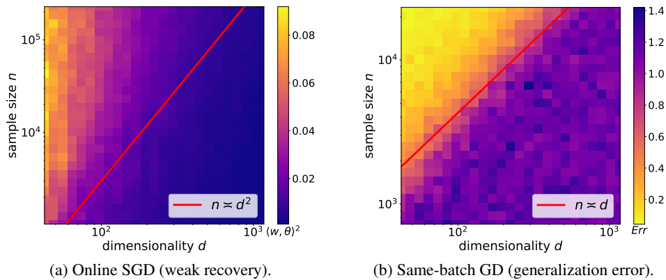
Figure 1: We train a ReLU NN (3.1) with N = 1024 neurons using SGD (squared loss) with step size \eta = 1/d to learn a single-index target f_*(\mathbf{x}) = \text{He}_3(\langle \mathbf{x}, \boldsymbol{\theta} \rangle) ; heatmaps are values averaged over 10 runs. (a) online SGD with batch size B = 8 ; (b) GD on the same batch of size n for T = 2^{14} steps. For online SGD we only report weak recovery (i.e., averaged overlap between neuron \mathbf{w} and target \boldsymbol{\theta} ) since the test error does not drop.
