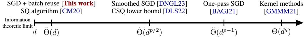
Figure 2: Complexity of learning single-index model where the link function \sigma_* is a degree- q polynomial with information exponent p . For the CSQ lower bound, we translate the tolerance to sample complexity using the i.i.d. concentration heuristic \tau \approx n^{-1/2} . We restrict ourselves to algorithms using polynomial compute; this excludes the sphere-covering procedure in [DPVLB24] or exponential-width neural network in [Bac17, TS24].
