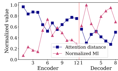
Figure 6: MAE properties.
