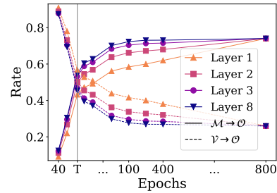
Figure 4: Exploitation rate.
