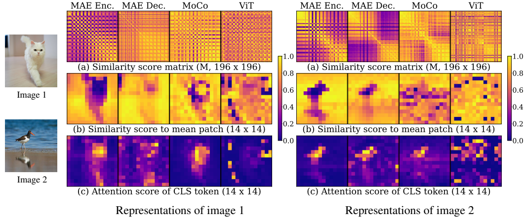
Figure 2: Relationships among the patch embeddings. (a) Pairwise similarity matrix for all 196 \times 196 pairs of patches. (b) Similarity between the mean patch and all individual patches. (c) Attention score of the class token.
