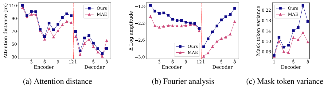
Figure 7: Metrics explaining our performance gain. Layers left on the red dotted line belong to the encoder, and the rest to the decoder.
