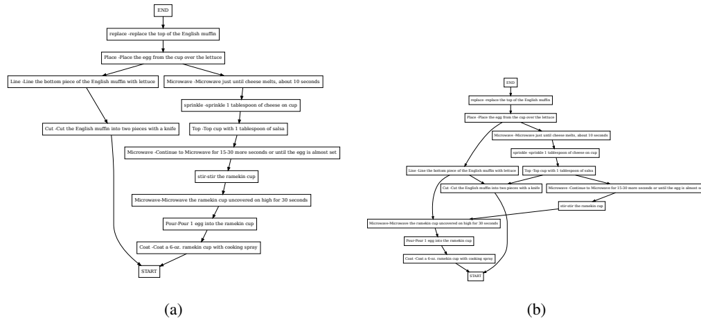
Figure 19: (a) Ground truth task graph and (b) predicted task graph of the scenario Microwave Egg Sandwich.
