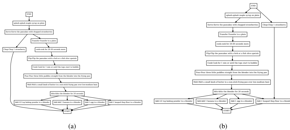
Figure 8: (a) Ground truth task graph and (b) predicted task graph of the scenario Breakfast Burritos.
