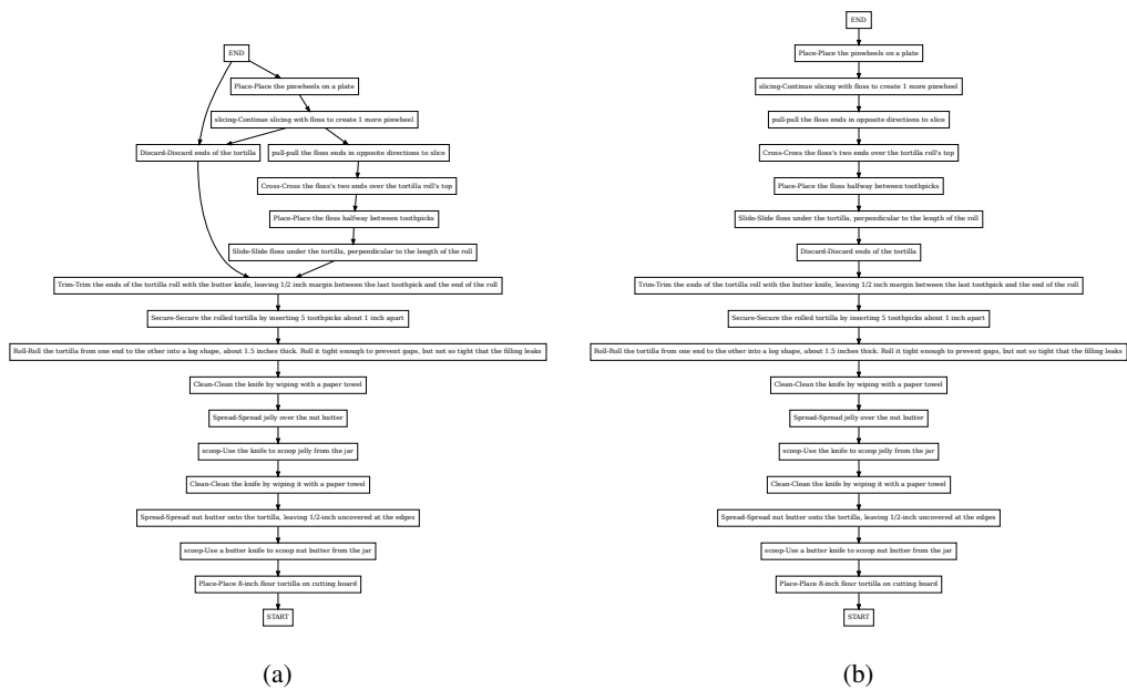
Figure 23: (a) Ground truth task graph and (b) predicted task graph of the scenario Pinwheels.
