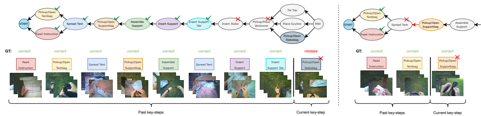
Figure 7: A success (left) and failure (right) case on EPIC-Tent-O. Past key-steps' colors match nodes' colors. On the left, the current key-step "Pickup/Open Stakebag" is correctly evaluated as a mistake because the step "Pickup/Place Ventcover" is a precondition of the current key-step, but it is not included among the previous key-steps. On the right, "Pickup/Open Supportbag" is incorrectly evaluated as mistake because the step "Spread Tent" is precondition of the current key-step, but it is not included among the previous key-steps. This is due to the fact that our method wrongly predicted "Spread Tent" as a pre-condition of "Pickup/Open Supportbag", probably due to the two actions often occurring in this order.
