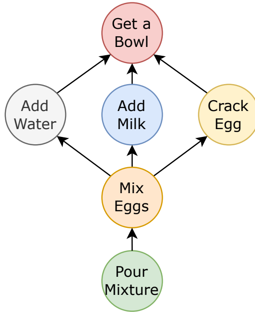
Figure 5: Example of a task graph where each node represents a key-step in the procedure, with directed edges indicating the necessary preconditions for each step.
