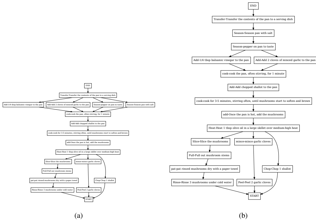
Figure 27: (a) Ground truth task graph and (b) predicted task graph of the scenario Salted Mushrooms.
