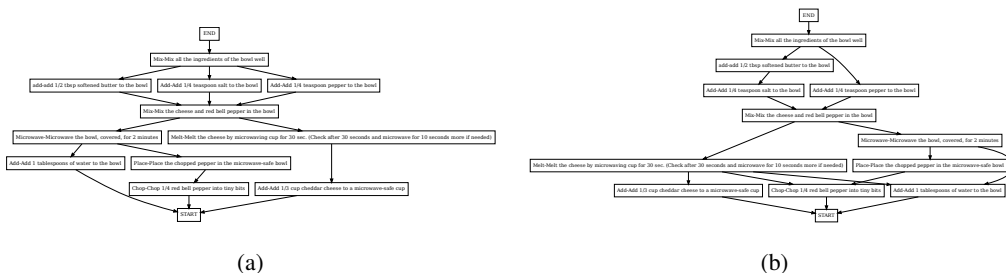
Figure 10: (a) Ground truth task graph and (b) predicted task graph of the scenario Cheese Pimiento.
