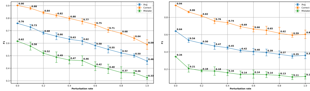
Figure 4: To further investigate the effect of noise, we conducted an analysis based on the controlled perturbation of ground truth action sequences, with the aim to simulate noise in the action detection process. At inference, we perturbed each key-step with a probability \alpha (the “perturbation rate”), with three kinds of perturbations: insert (inserting a new key-step with a random action class), delete (deleting a key-step), or replace (randomly changing the class of a key-step). The plots show the trend of the F1 score (Average, Correct, and Mistake) as the perturbation rate increases in the case of Assembly101-O (left) and EPIC-Tent-O (right). Results suggest that the proposed approach can still bring benefits even in the presence of imperfect action detections, with the average F1 score dropping down 10 – 15 points with a moderate noise level of 20%.
