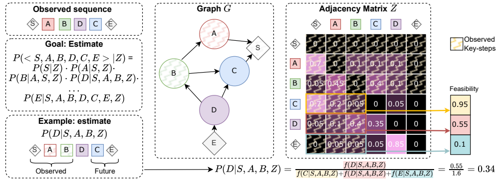
Figure 2: Given a sequence \langle S, A, B, D, C, E \rangle , and a graph G with adjacency matrix Z , our goal is to estimate the likelihood P(\langle S, A, B, D, C, E \rangle | Z) , which can be done by factorizing the expression into simpler terms. The figure shows an example of computation of probability P(D | S, A, B, Z) as the ratio of the “feasibility of sampling key-step D, having observed key-steps S, A, and B” to the sum of all feasibility scores for unobserved symbols. Feasibility values are computed by summing weights of edges D \rightarrow X for all observed key-steps X .
