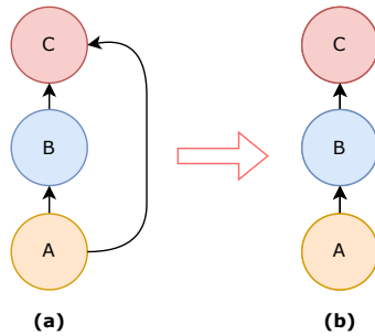
Figure 6: An example of transitive dependency between nodes. In (a) node A depends on B and C, but B depends on C, in this case, we can remove the edge between A and C for transitivity and we obtain the graph in (b).
