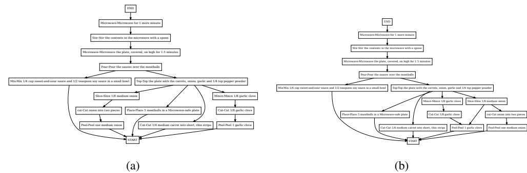
Figure 13: (a) Ground truth task graph and (b) predicted task graph of the scenario Dressed Up Meatballs.
