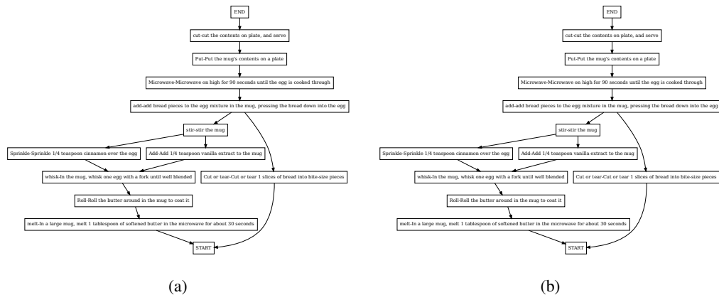
Figure 20: (a) Ground truth task graph and (b) predicted task graph of the scenario Microwave French Toast.
