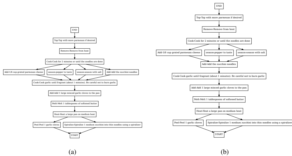
Figure 16: (a) Ground truth task graph and (b) predicted task graph of the scenario Zoodles.
