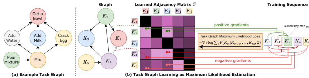
Figure 1: (a) An example task graph encoding dependencies in a “mix eggs” procedure. (b) We learn a task graph which encodes a partial ordering between actions (left), represented as an adjacency matrix Z (center), from input action sequences (right). The proposed Task Graph Maximum Likelihood (TGML) loss directly supervises the entries of the adjacency matrix Z generating gradients to maximize the probability of edges from past nodes ( K_3, K_1 ) to the current node ( K_2 ), while minimizing the probability of edges from past nodes to future nodes ( K_4, K_5 ) in a contrastive manner.
