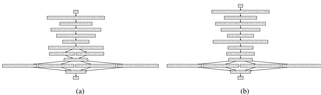
Figure 17: (a) Ground truth task graph and (b) predicted task graph of the scenario Microwave Mug Pizza.
