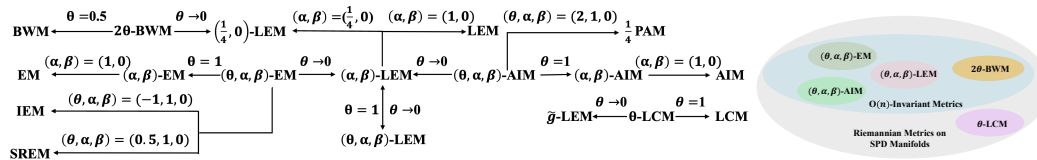
Figure 1: Illustration on the deformation (left) and Venn diagram (right) of metrics on SPD manifolds, where IEM, SREM, and \frac{1}{4} PAM denotes Inverse Euclidean Metric, Square Root Euclidean Metric, and Polar Affine Metric scaled by 1/4 .
