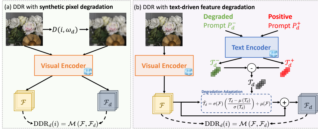
Figure 3: The framework of our proposed DDR with two different degradation fusing methods. (a) Synthesizing degradation with a handcrafted process in the pixel domain. (b) Fusing text-driven degradation in the feature domain.
