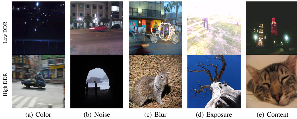
Figure 4: Images with high and low DDR to different degradation types. We measure DDR with five types of degradation by setting their corresponding prompt pair. We observe that image with lower DDR to a specific type of degradation is likely to obtain this degradation of a higher level.
