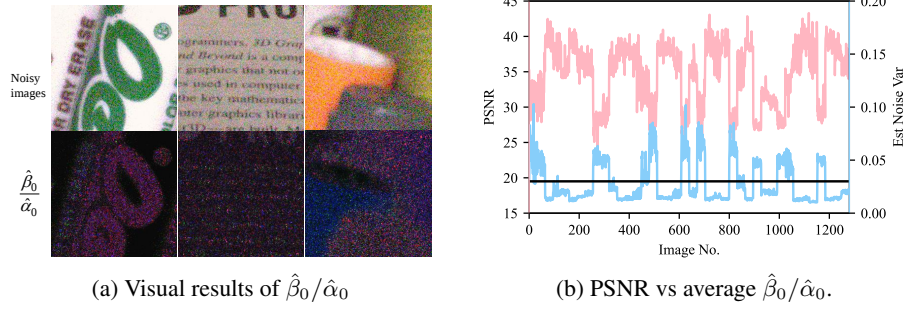
Figure 4: The estimated noise variance 1/E(\phi_0) = \hat{\beta}_0/\hat{\alpha}_0 on SIDD dataset
