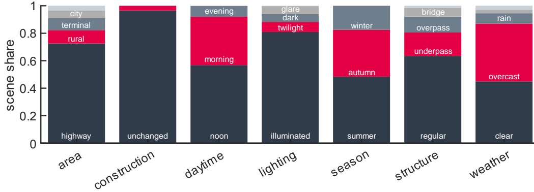
Figure 3: Distribution of the scene tags for all 747 dataset scenes.
