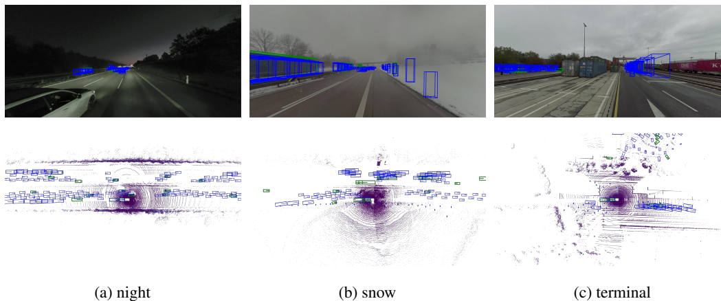
Figure A12: Example visualizations of the PETR model on the validation split of the MAN TruckScenes dataset v1.0. The front left camera is shown on the top and the fused lidar point cloud on the bottom. Model predictions are shown in blue and the ground truth in green.
