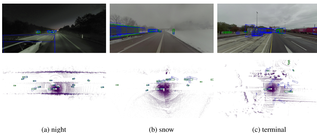
Figure A13: Example visualizations of the RadarGNN model on the validation split of the MAN TruckScenes dataset v1.0. The front left camera is shown on the top and the fused lidar point cloud on the bottom. Model predictions are shown in blue and the ground truth in green.
