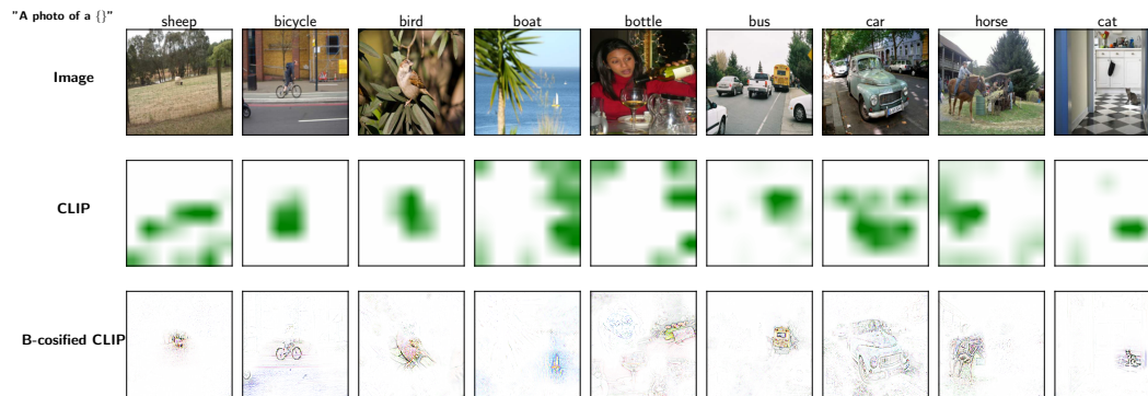
Fig. 2: B-cosified CLIP Models. After B-cosifying a CLIP model and fine-tuning it according to our proposed B-cosification scheme, see Sec. 3.2, we find that it is possible to endow the model with the same level of inherent interpretability as the B-cos models proposed in [11], whilst maintaining CLIP’s zeroshot ability (see Fig. 5). The resulting linear summaries of the models ( \mathbf{W}(\mathbf{x}) ) can be visualised in color (row 3) and provide significantly more detail than GradCAM explanations (row 2), which are often used to explain conventional CLIP models.
