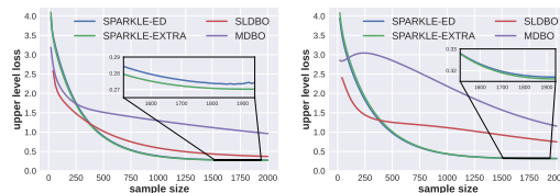
Figure 3: The upper-level loss against samples generated by one agent of different algorithms in the policy evaluation. (Left: n = 10 , Right: n = 20 .)
