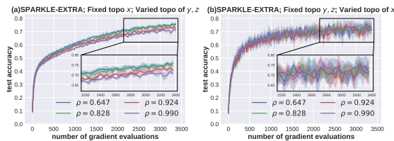
Figure 2: Test accuracy of SPARKLE-EXTRA on hyper-cleaning. (Left: fixed graph for x and varying graph for y, z ; Right: fixed for y, z and varying for x )
