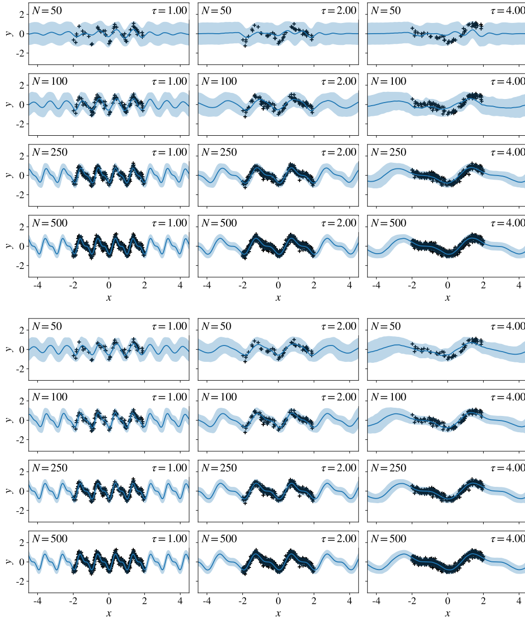
Figure S4: Example model fits for the DPConvCNP on the sawtooth task. For all the above fits, a single amortised DPConvCNP is used, that is a DPConvCNP that has been trained on sawtooth data with randomly chosen periods \tau^{-1} \sim \mathcal{U}[0.20, 1.25] and random privacy budgets, specifically \epsilon \sim \mathcal{U}[0.90, 4.00] and \delta = 10^{-3} . The first four rows correspond to \epsilon = 1.00 and the last four to \epsilon = 3.00 . We have fixed \delta = 10^{-3} . Note that column-wise the datasets are fixed, and we are varying the context set size N .
