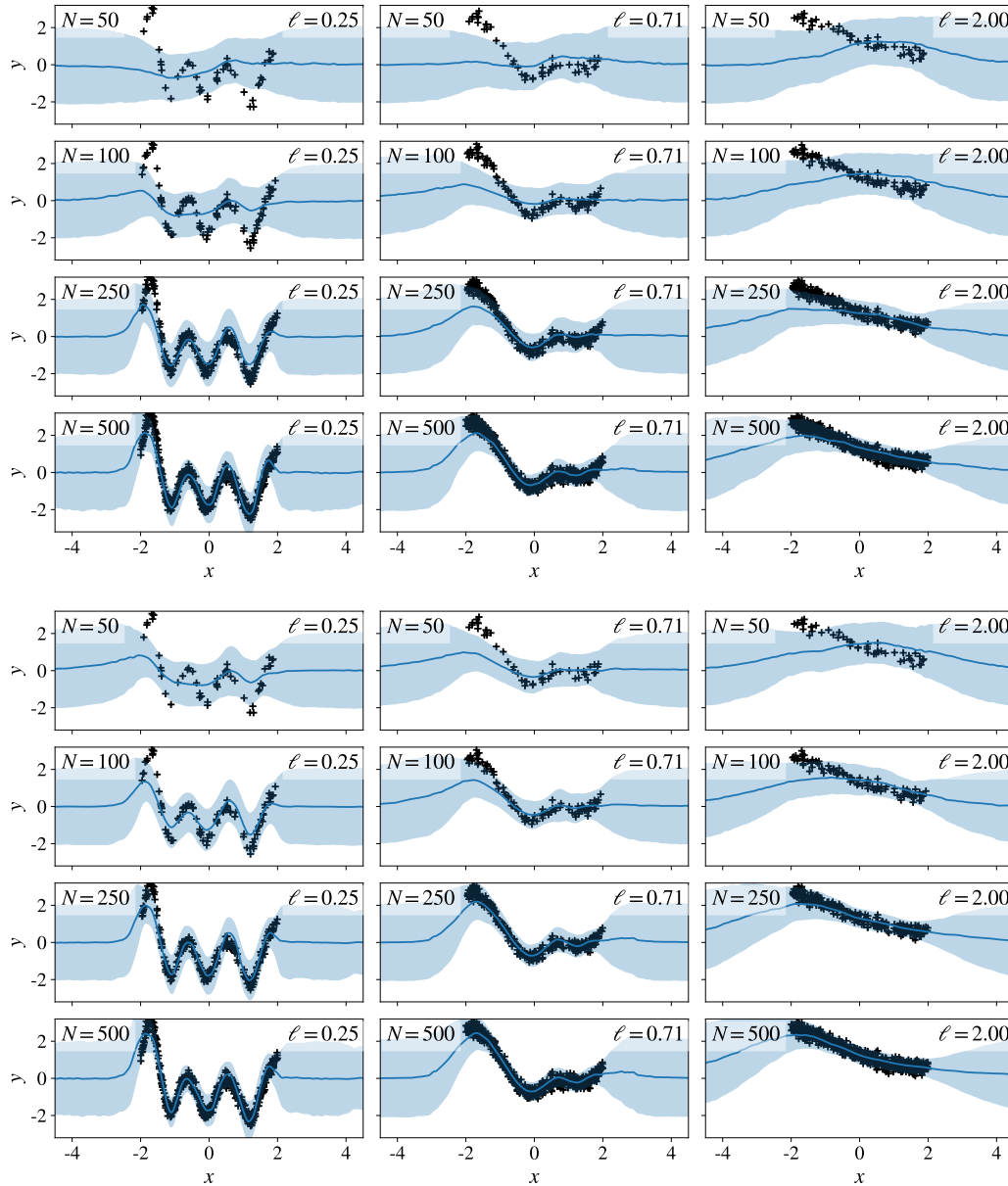
Figure S3: Same as Figure S2, but with a different dataset seed. Example model fits for the DPConvCNP on the EQ GP task. For all the above fits, a single amortised DPConvCNP is used, that is a DPConvCNP that has been trained on EQ GP data with randomly chosen lengthscales \ell \sim \mathcal{U}[0.20, 2.50] and random privacy budgets, specifically \epsilon \sim \mathcal{U}[0.90, 4.00] and \delta = 10^{-3} . The first four rows correspond to \epsilon = 1.00 and the last four to \epsilon = 3.00 . We have fixed \delta = 10^{-3} . Note that column-wise the datasets are fixed, and we are varying the context set size N .
