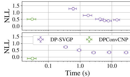
Figure 5: Deployment-time comparison on Gaussian (top) and non-Gaussian (bottom) data. We ran the DP-SVGP for different numbers of DP-SGD steps to determine a speed versus quality-of-fit tradeoff. Reporting 95% confidence intervals.
