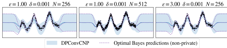
Figure 2: Training our proposed model with a DP mechanism inside it, enables the model to make accurate well-calibrated predictions, even for modest privacy budgets and dataset sizes. Here, the context data (black) are protected with different (\epsilon, \delta) DP budgets as indicated. The model makes predictions (blue) that are remarkably close to the optimal (non-private) Bayes predictor.
