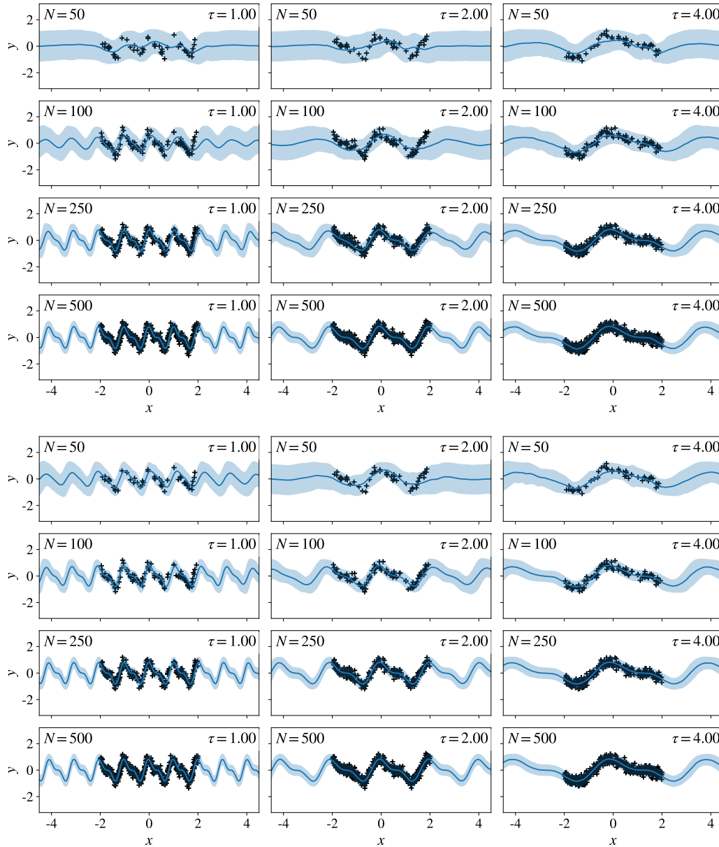
Figure S5: Same as Figure S4, but with a different dataset seed. Example model fits for the DPConvCNP on the sawtooth task. For all the above fits, a single amortised DPConvCNP is used, that is a DPConvCNP that has been trained on sawtooth data with randomly chosen periods \tau^{-1} \sim \mathcal{U}[0.20, 1.25] and random privacy budgets, specifically \epsilon \sim \mathcal{U}[0.90, 4.00] and \delta = 10^{-3} . The first four rows correspond to \epsilon = 1.00 and the last four to \epsilon = 3.00 . We have fixed \delta = 10^{-3} . Note that column-wise the datasets are fixed, and we are varying the context set size N .
