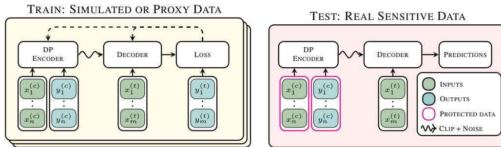
Figure 1: Meta-training (left) and meta-testing (right) using our method. We train a model on multiple tasks with non-private (simulated or proxy) data to predict on target ( t ) points using the context ( c ) points. Crucially, by including a DP mechanism, which clips and adds noise to the data during training , the parameter updates (dashed arrow) teach the model to make well-calibrated and accurate predictions in the presence of DP noise. At test time, we deploy the model on real data using the same mechanism, which protects the context set with DP guarantees.
