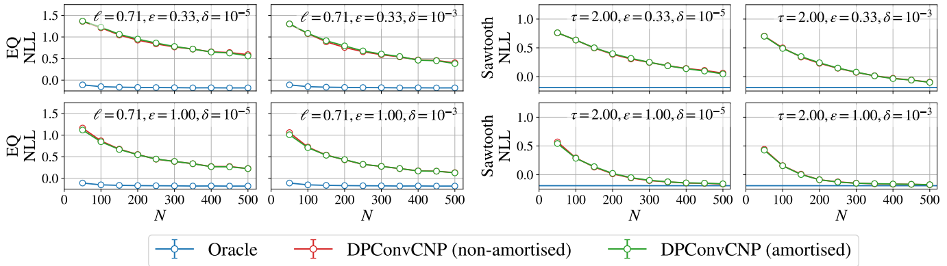
Figure S6: Additional results using the DPCovCNP on the EQ and sawtooth synthetic tasks with stricter DP parameters, namely all combinations of \epsilon = \{1/3, 1\} and \delta = \{10^{-5}, 10^{-3}\} . The overall setup in this figure is identical to that in Figure 6, except the amortised DPCovCNP is trained on randomly chosen \epsilon \sim \mathcal{U}[1/3, 1] and fixed \delta = 10^{-5} or 10^{-3} , and the non-amortised DPCovCNP models are trained on \epsilon and \delta values as indicated on the plots. Then, both amortised and non-amortised models are evaluated with the parameters shown on the plots. The DP-SVGP baseline was not run due to time constraints in the rebuttal period: it is significantly slower and more challenging to optimise than the DPCovCNP. We note that the amortisation gap, due to training a model to handle a continuous range of \epsilon values, is negligible. We also note that as the number of context points N increases, the performance of the DPCovCNP approaches that of the oracle predictors.
