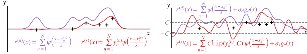
Figure 3: Left; Illustration of the ConvCNP encoder \text{enc}_\phi . Black crosses show an example context set D^{(c)} . The density channel r^{(d)} is shown in purple and the signal channel r^{(s)} is shown in red. The representation r consists of concatenating r^{(d)} and r^{(s)} . Right; Illustration of the DPConvCNP encoder. Black crosses show an example context D^{(c)} , clipped with a threshold C (gray dashed). Here, a single point (rightmost) is clipped (gray cross shows value before clipping). The density and signal channels are computed and GP noise is added to obtain the DP representation (red & purple).
