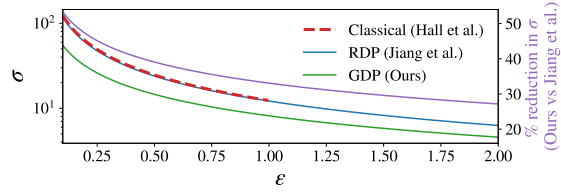
Figure 4: Noise magnitude comparison for the classical functional mechanism of Hall et al. [2013], the RDP-based mechanism of Jiang et al. [2023] and our improved GDP-based mechanism. The line for Hall et al. cuts off at \epsilon = 1 since their bound has only been proven for \epsilon \leq 1 . We set \Delta^2 = 10 and \delta = 10^{-3} , which are representative values from our experiments. See Appendix A.6 for more details.
