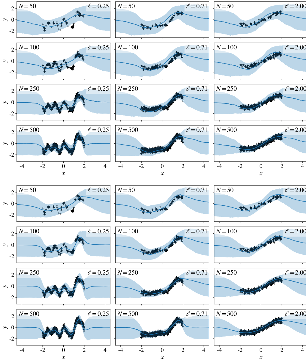
Figure S2: Example model fits for the DPConvCNP on the EQ GP task. For all the above fits, a single amortised DPConvCNP is used, that is a DPConvCNP that has been trained on EQ GP data with randomly chosen lengthscales \ell \sim \mathcal{U}[0.20, 2.50] and random privacy budgets, specifically \epsilon \sim \mathcal{U}[0.90, 4.00] and \delta = 10^{-3} . The first four rows correspond to \epsilon = 1.00 and the last four to \epsilon = 3.00 . We have fixed \delta = 10^{-3} . Note that column-wise the datasets are fixed, and we are varying the context set size N .
