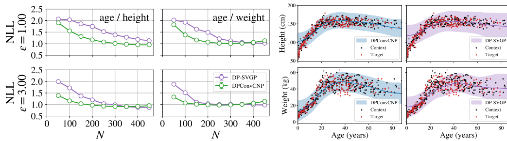
Figure 7: Left; Negative log-likelihoods of the DPConvCNP and the DP-SVGP baseline on the sim to real task with the !Kung dataset, predicting individuals’ height from their age (left col.) or their weight from their age (right col.). For each point shown here, we partition each dataset into a context and target at random, make predictions, and repeat this procedure 512 times. We report mean NLL with its 95% confidence intervals. Error bars are too small to see here. Right; Example predictions for the DPConvCNP and the DP-SVGP, showing the mean and 95% confidence intervals, with N = 300 , \epsilon = 1.00 , \delta = 10^{-3} . The DPConvCNP is visibly better-calibrated than the DP-SVGP.
