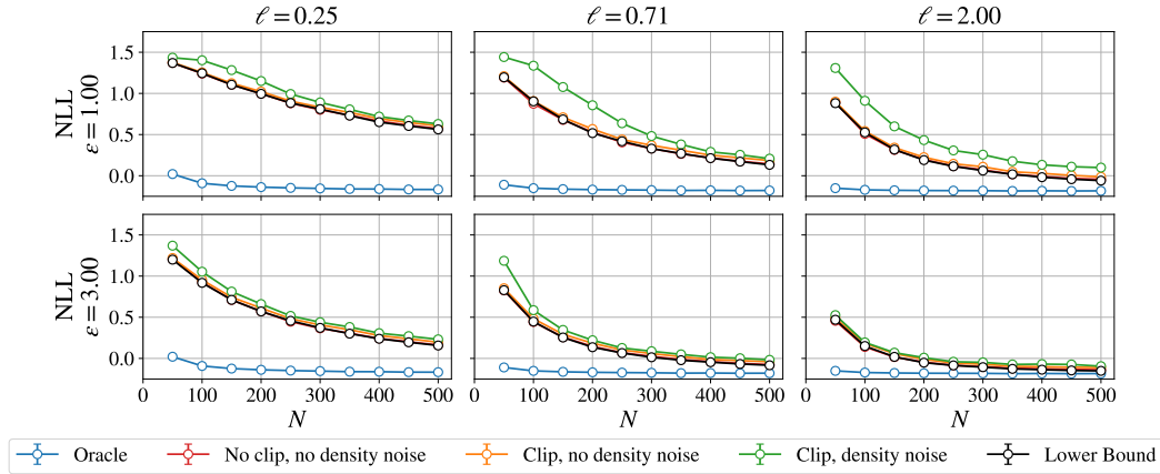
Figure S1: DPConvCNP performance on the GP modelling task, where the data are generated using an EQ GP with lengthscale \ell . We train three models per \epsilon, \ell combination, keeping \delta = 10^{-3} fixed as well as the clipping threshold C = 2.00 and noise weight t = 0.50 fixed. Specifically, we train one model where only noise to the signal channel (red; no clip, no density), one model where noise and clipping are applied to the signal channel (orange; clip, no density noise) and another model where noise and clipping to the signal channel as well as noise to the density channel are applied (green; clip, density noise). We also show the NLL of the oracle, non-DP, Bayesian posterior, which is the best average NLL that can be obtained on this task (blue). Lastly, we show a bound to the functional mechanism (black), which is a lower bound on the NLL that can be obtained with the functional mechanism with C = 2.00, t = 0.50 on this task. We used 512 evaluation tasks for each N, \ell, \epsilon combination, and report mean NLLs together with their 95% confidence intervals. Note that the error bars are plotted but are too small to see in the plot.
