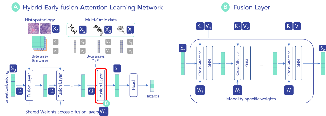
Figure 1: Overview of HEALNet ( H ybrid E arly-fusion A ttention L earning N etwork) using a shared and modality-specific parameter space to learn from structurally different data sources in the same model (Fig. 1A). The shared space is a learned latent embedding S that is iteratively updated through d attention-based fusion layers and captures the shared information between modalities. The hybrid early-fusion layer (Fig. 1B, and Eq. 3) learns the cross-attention weights W_m = \{W_m^{(q)}, W_m^{(k)}, W_m^{(v)}\} for each modality m corresponding to the queries ( Q_m = W_m^{(q)} S ), keys ( K_m = W_m^{(k)} X_m ), and values ( V_m = W_m^{(v)} X_m ) which are shared between layers. These layers capture the structural information of each modality and encode it in the shared embedding after a pass through a self-normalising network (SNN) layer.
