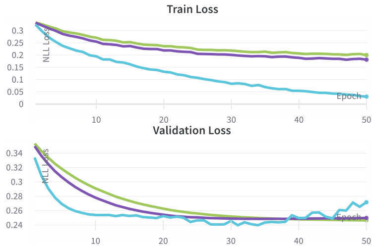
Figure 4: Effect of the regularisation mechanism. We show the train (top) and validation (bottom) losses on the KIRP dataset, of HEALNet variants with no regularisation (blue), only L1 regularisation (indigo), and L1 regularisation + a self-normalising network layer (green).
