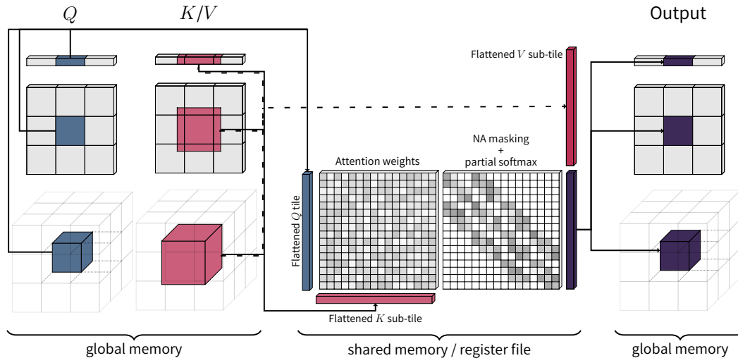
Figure 4: A simplified illustration of fused neighborhood attention. Q and KV tensors are tiled according to their spatial layout (1-D, 2-D, 3-D), with the latter haloed to include the entire neighborhood for all corresponding queries in the query tile. Resulting attention weights from the first GEMM are masked according to neighborhood attention parameters, before undergoing online softmax scaling, and going through the second GEMM with the corresponding value sub-tile.
