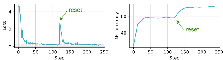
Figure 5: Training loss curve and multiple choice performance during training with active forgetting, on the Narrative text of Country-city-animals, LLaMA 3 8B. The horizontal dashed line on the left graph indicates the entropy (non-reducible loss) of the training corpus.
