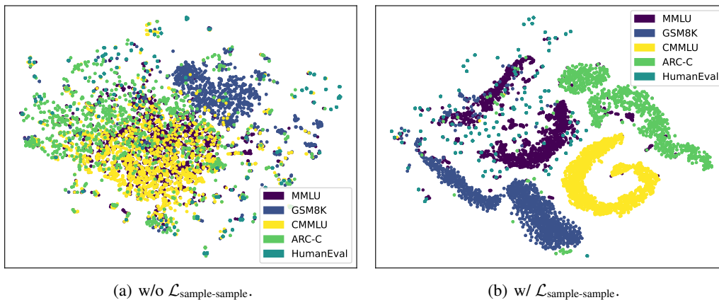
Figure 15: t-SNE visualization of training query embeddings extracted by the learned encoder.
