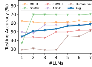
Figure 13: Testing accuracy with different numbers of LLMs.
