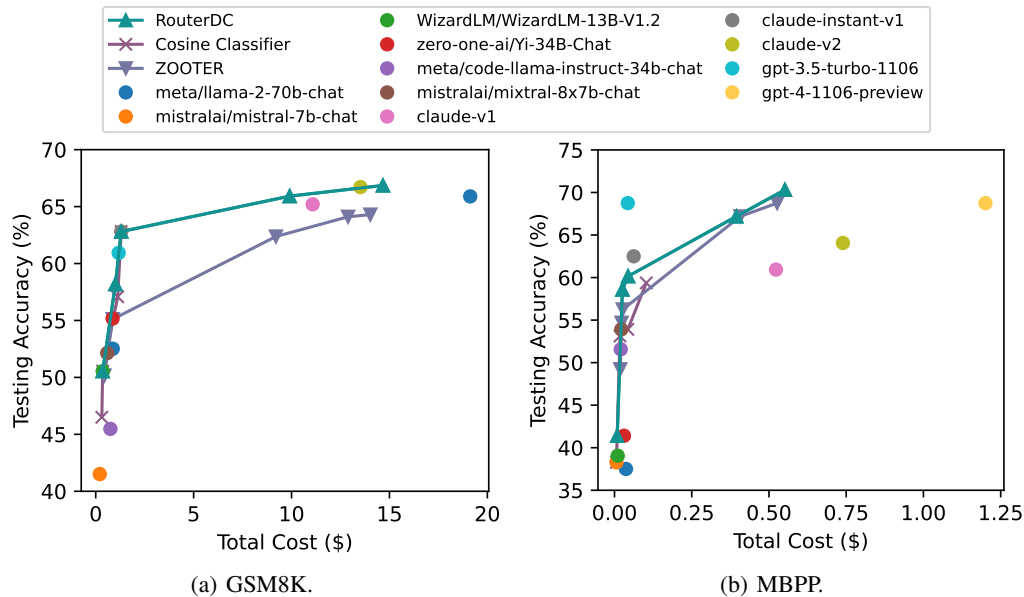
Figure 14: Testing accuracy with different costs on RouterBench.
