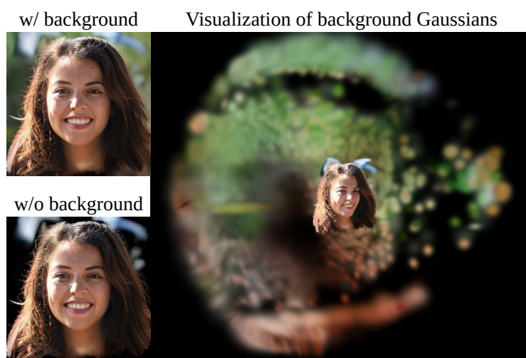
Figure 15: Visualization of effects of background generator
