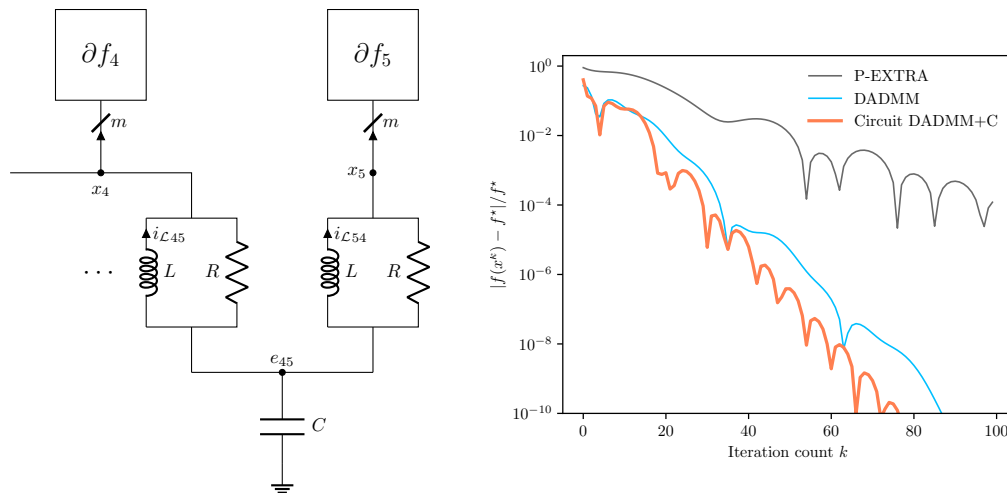
Figure 9: (Left) Circuit of DADMM+C. Compared to the DADMM circuit of §F.3, the DADMM+C circuit has an additional capacitor. (Right) Relative error |f(x^k) - f^*| / f^* vs. iteration count k .
