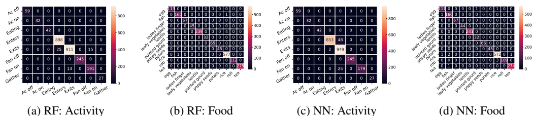
Figure 13: Confusion Matrix of indoor activity and food item classification with (a)(b) Random Forest with max estimators 50 and max depth 10, (c)(d) Neural Network with three 64-neuron hidden layer.
