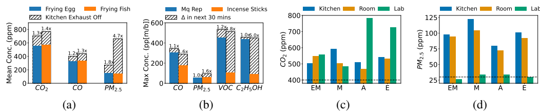
Figure 5: (a) depicts pollutant accumulation if the kitchen exhaust fan is turned off (i.e., 4.7 \times PM_{2.5} ). (b) shows the maximum pollutant increase before and after 30 minutes of using mosquito repellent (Mq Rep) or burning incense sticks (i.e., 4.8 \times VOC for burning sticks). Further, we have divided the day into Early Morning (EM, 00:00–06:00), Morning (M, 06:00–12:00), Afternoon (A, 12:00–18:00), and Evening (E, 18:00–23:00) hours. (c) shows in the morning, the kitchen has higher CO_2 , while research labs are impacted in the afternoon and evening due to occupancy. Lastly, (d) shows that PM_{2.5} is predominant in the kitchen and rooms at any time of the day. The dashed line represents healthy pollutant level.
