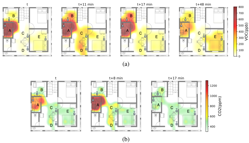
Figure 14: Spatiotemporal spread of – (a) VOC, and (b) CO 2 from the kitchen in Household H1. The figure is reproduced to provide insights on the dataset and depicted in work [50].
