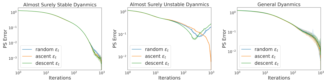
Figure 1: PS Error \|\mathbf{M}_N - \mathbf{M}^{PS}\|_F^2
