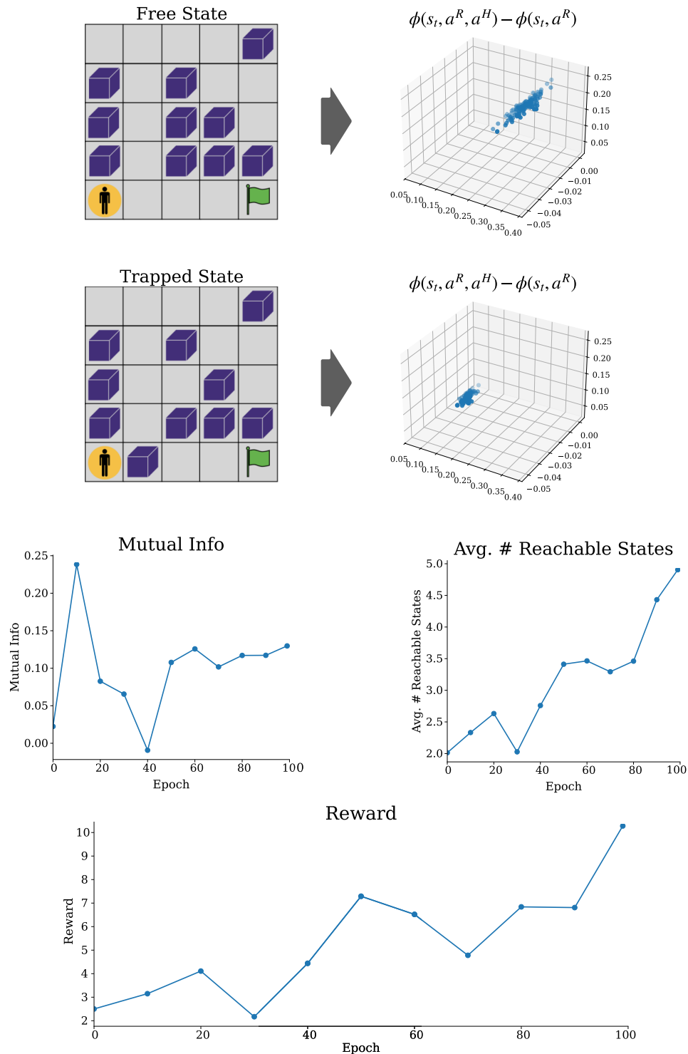
Figure 8: Visualizing training empowerment in a 5x5 Gridworld with 10 obstacles. Our empowerment objective maximizes the influence of the human's actions on the future state, preferring the state where the human can reach the goal to the trapped state. This corresponds to maximizing the volume of the state marginal polytope, which is proportional to the number of states that the human can reach from their current position. To visualize the representations, we set the latent dimension to 3 instead of 100.
