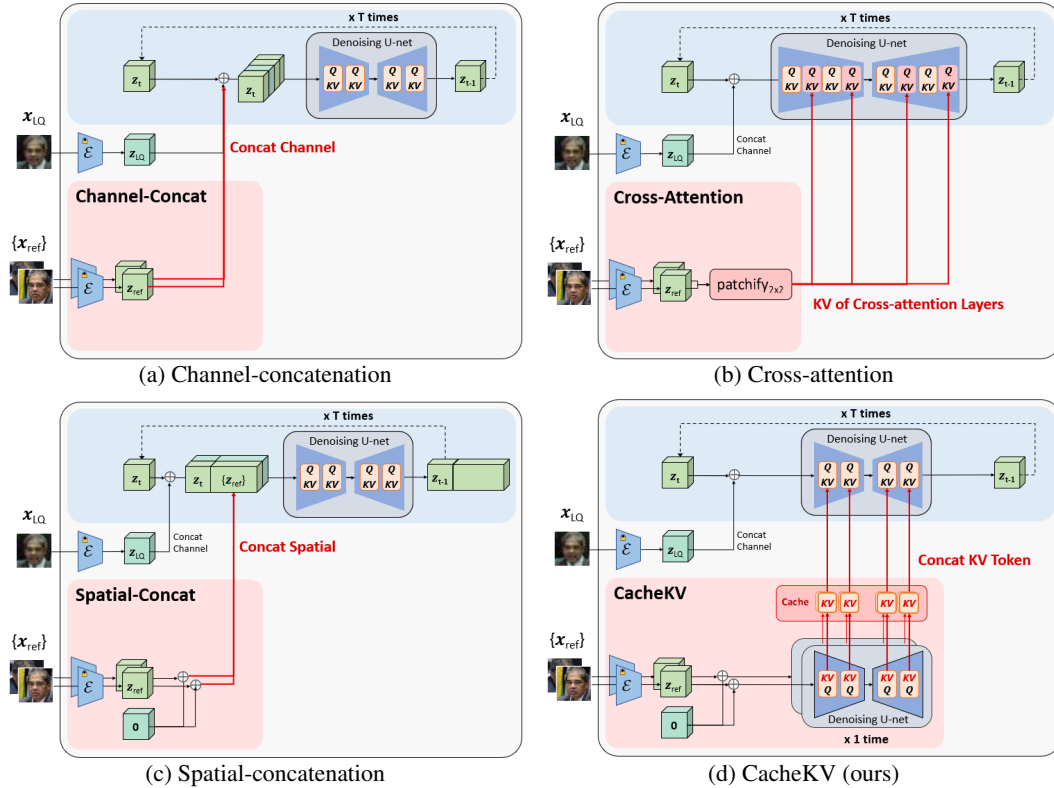
Figure 3: Different mechanisms for incorporating reference images into the main denoising process.
